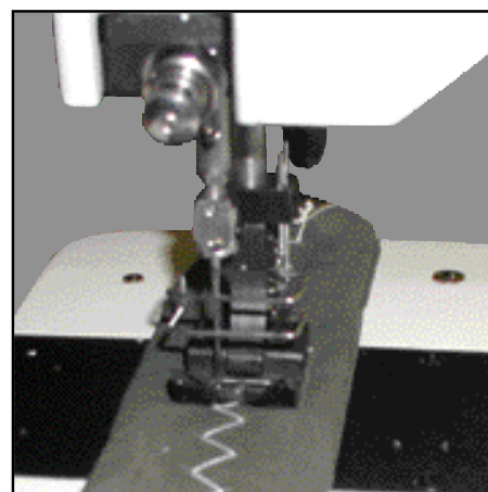
Extra wide zig-zag (12.7mm) even under heavy loads
