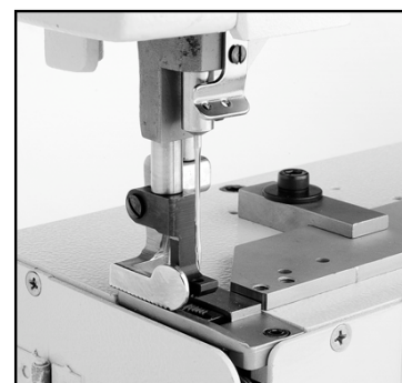
Walking foot with built-in edge guide
