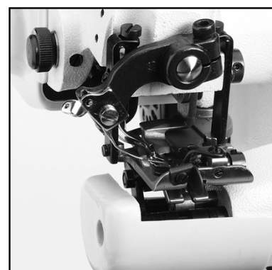
Swing down cylinder arm
