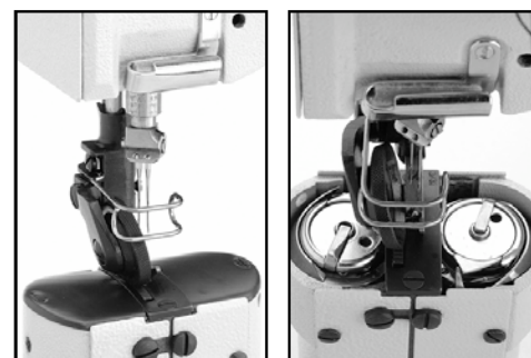
Large roller foot Standard vertical hooks
